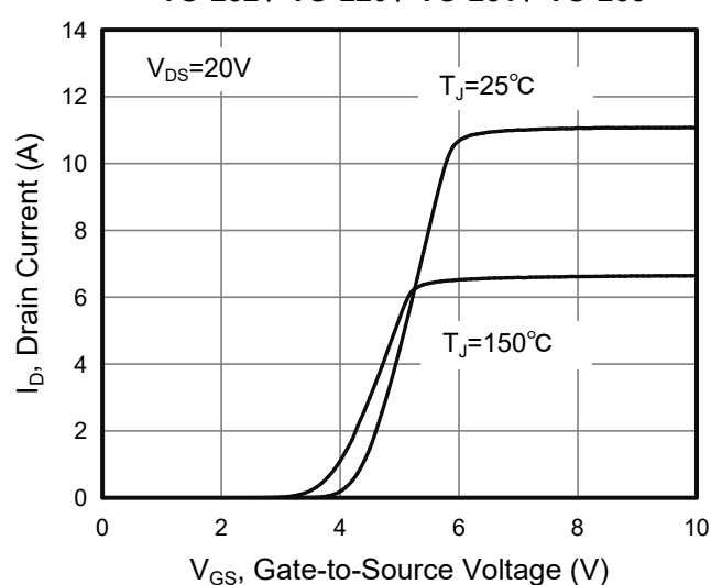
Figure 6. Transfer Characteristics
