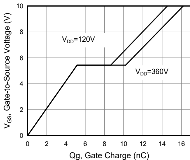
Figure 9. Gate Charge
