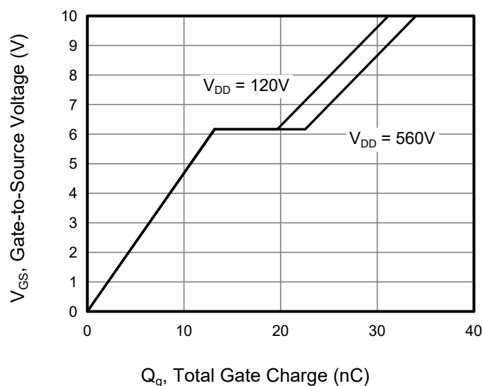
Figure 9. Gate Charge
