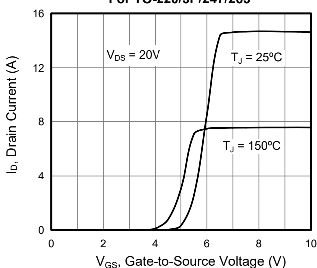
Figure 6. Transfer Characteristics
