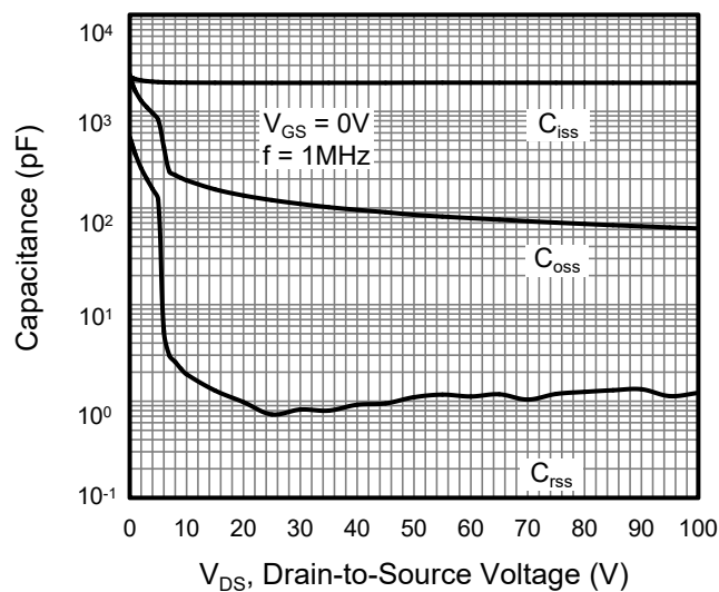
Figure 8. Capacitance
