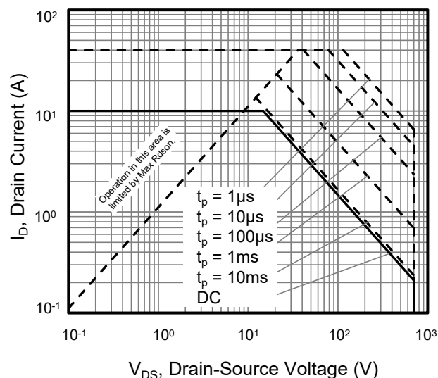
Figure 3. Safe Operation Area For TO-220/3P/247/263
