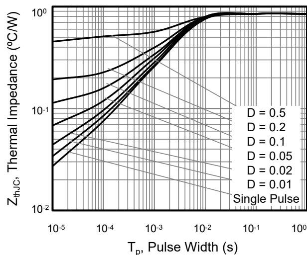
Figure 1. Transient Thermal Impedance For TO-220/3P/247/263
