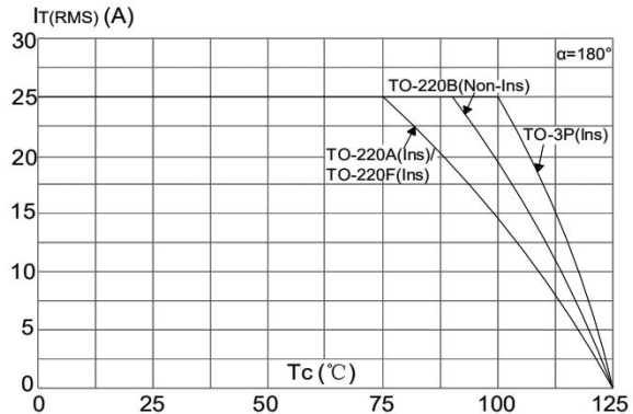
FIG.2: on-state current versus case temperature
