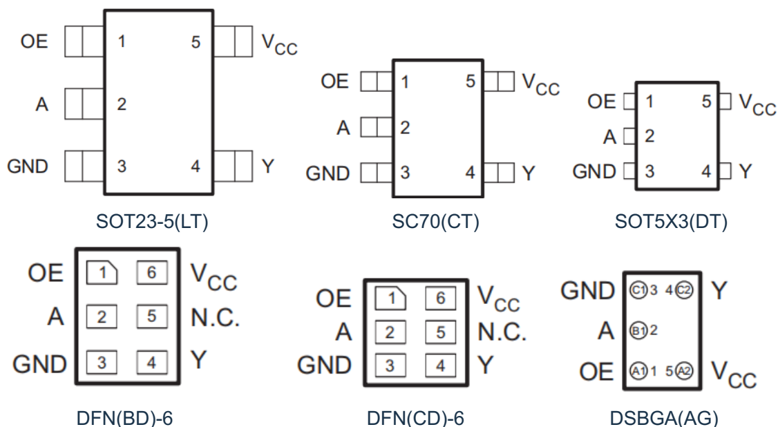
Figure 2.1: Top View
