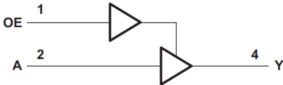
Figure 3.1: 74LVC1G126 Logic Diagram
