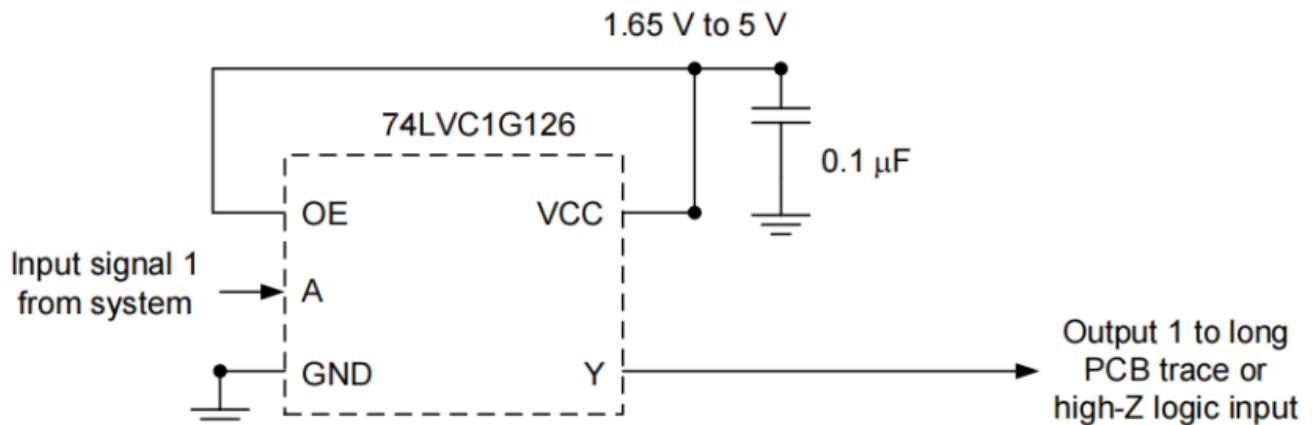
Figure 5.1: Application Schematic
