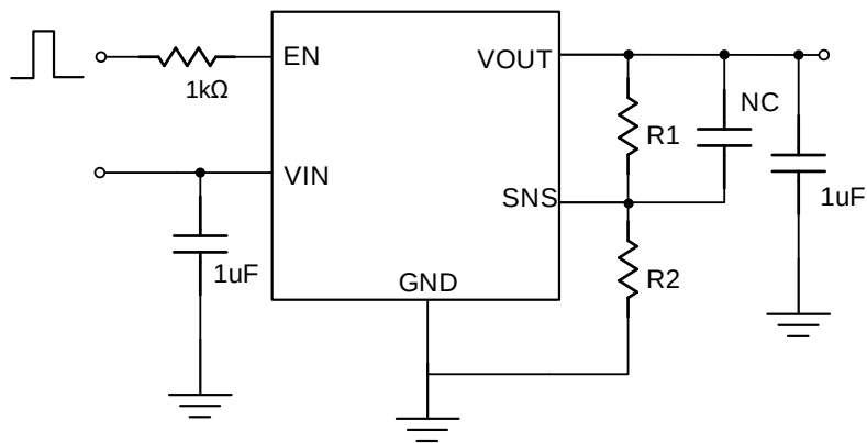
Figure 2: Adjustable output voltage LDO application circuit by DS8403N
