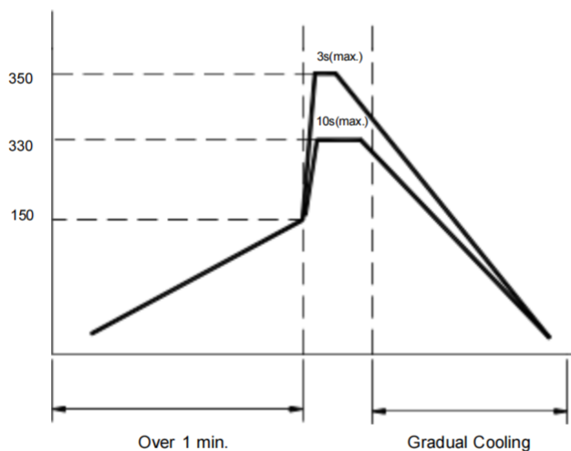
Figure 3. Hand Soldering
