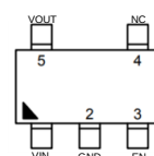
SC-70-5
