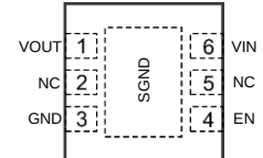
DFN2x2-6L
