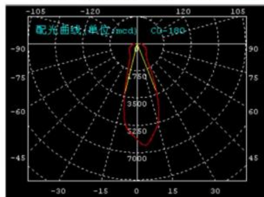
Light intensity distribution curve
