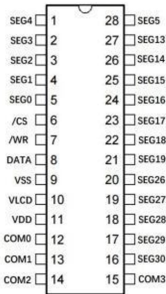
HTM1621- TD 28SOP-A/SSOP-A
