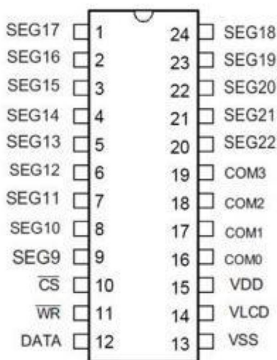
HTM1621- TD 24SOP-A/SSOP-A
