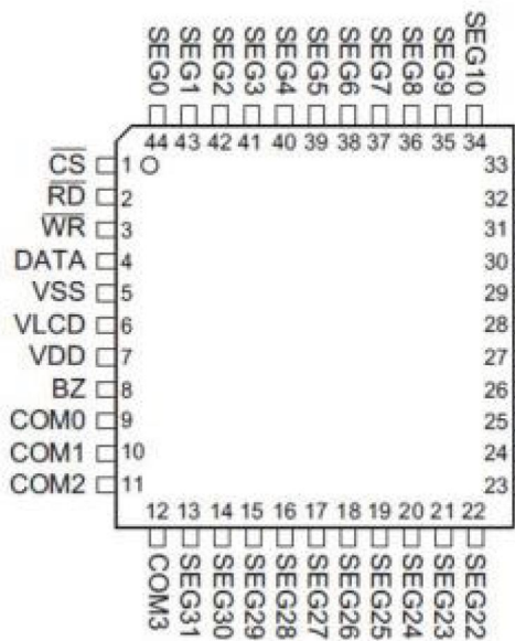
HTM1621- TD 44LQFP-A
