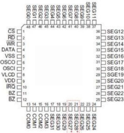
HTM1621-TD 48LQFP-A
