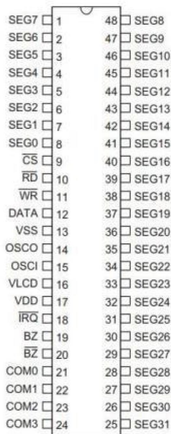
HTM1621- TD 48SSOP-A
