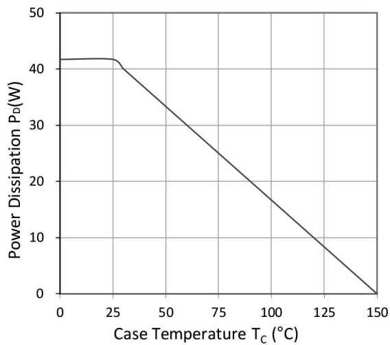
Figure 9. Power Dissipation
