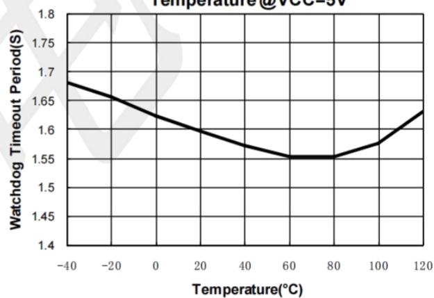
Watchdog Timeout Period vs. Temperature@VCC=5V
