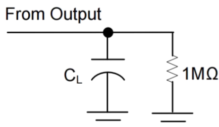
TEST CIRCUIT
