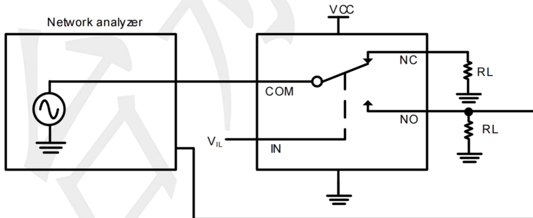
Off isolation
