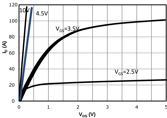
Fig 1: Output Characteristics
