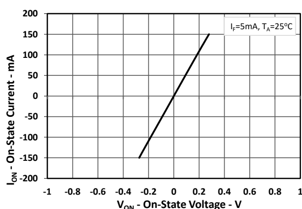
Fig. 3 On-State Current vs. On-State Voltage
