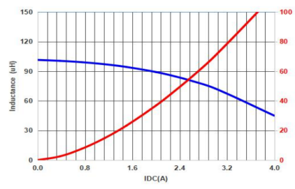
MMPC1005-101MT
