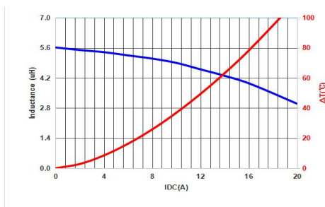
MMPC1005-5R6MT
