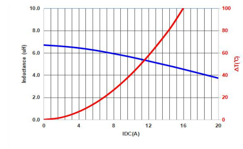
MMPC1005-6R8MT
