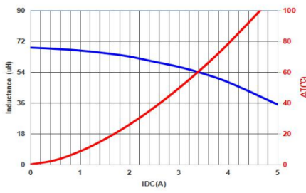
MMPC1005-680MT
