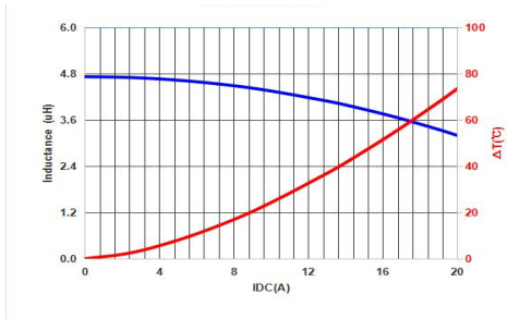
MMPC1005-4R7MT
