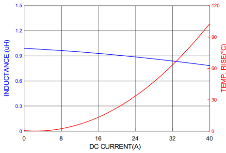
MMPC1235-1R0MT
