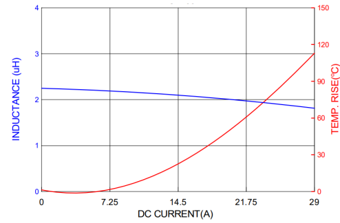
MMPC1235-5R6MT
