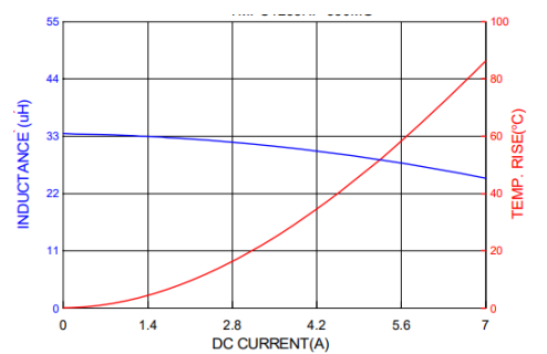
MMPC1235-330MT
