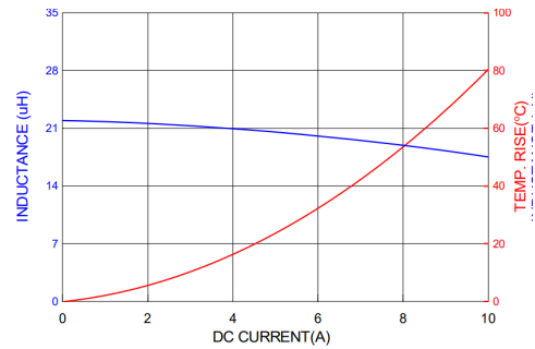
MMPC1235-220MT
