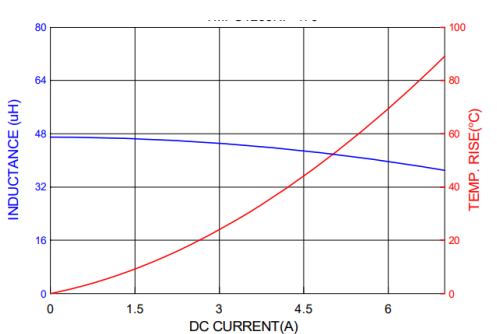
MMPC1235-470MT
