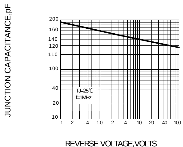
FIG.5 – PEAK JUNCTION CAPACITANCE
