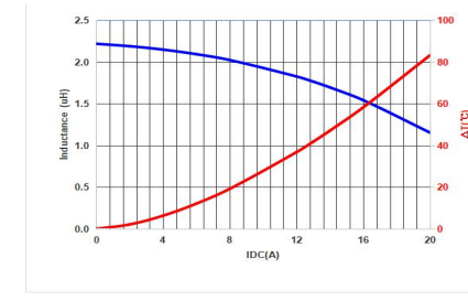
MMPC1003-5R6MT
