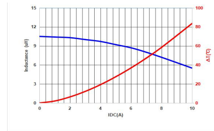
MMPC1003-100MT
