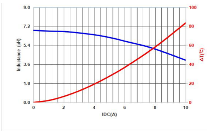
MMPC1003-8R2MT
