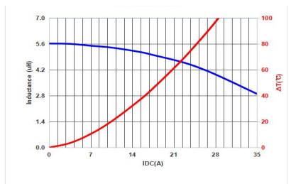
MMPC1206-5R6MT
