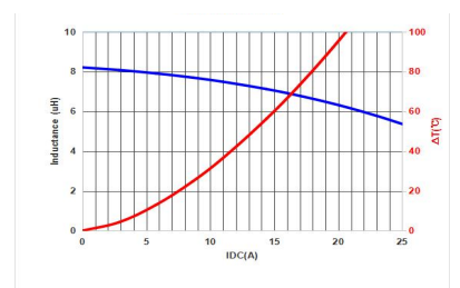
MMPC1206-8R2MT
