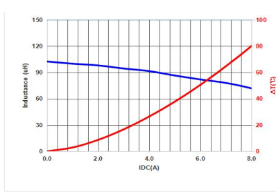
MMPC1206-171MT
