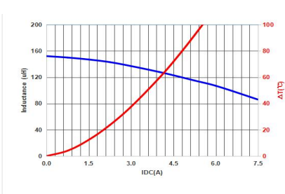
MMPC1206-151MT
