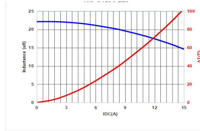
MMPC1206-560MT
