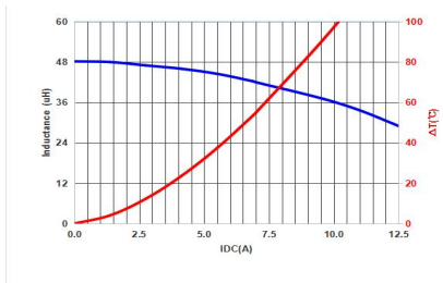
MMPC1206-820MT
