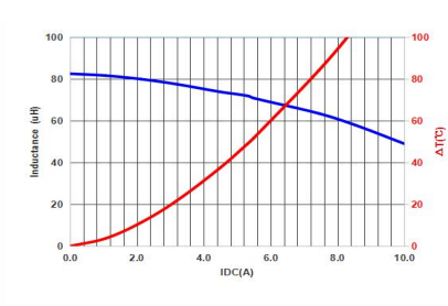
MMPC1206-151MT
