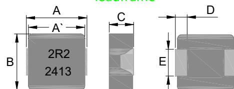
non-leadframe
