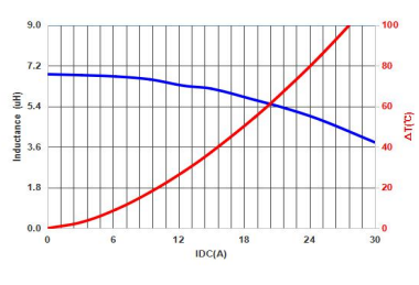
MMPC1205-6R8MT
