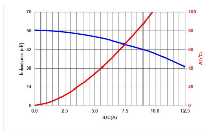
MMPC1206-101MT
