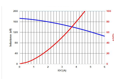
MMPC1206-171MT
