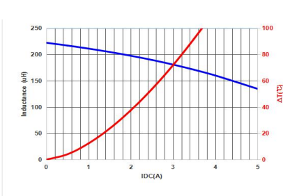
MMPC1206-221MT
