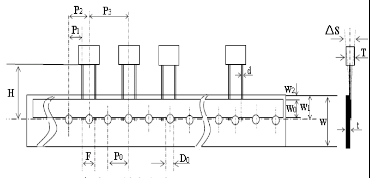
Fig.2 P=10.0/15.0mm
