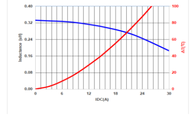
MMPC0602-R68MT
