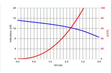
MMPC0602-150MT
