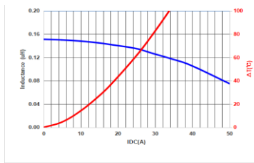
MMPC0602-R47MT
