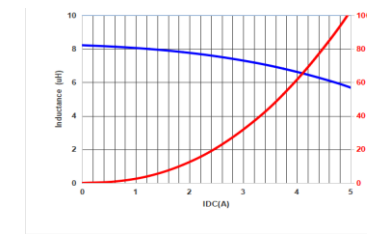
MMPC0602-220MT
