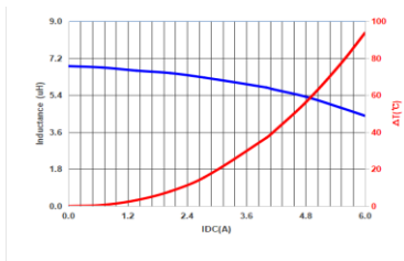
MMPC0602-150MT
