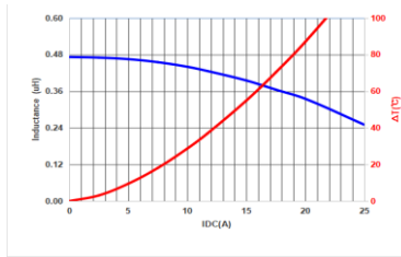
MMPC0602-1R0MT
