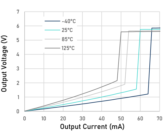
Output Voltage Swing as a function of Output Current (Sinking, V_S = 40\text{ V} )
