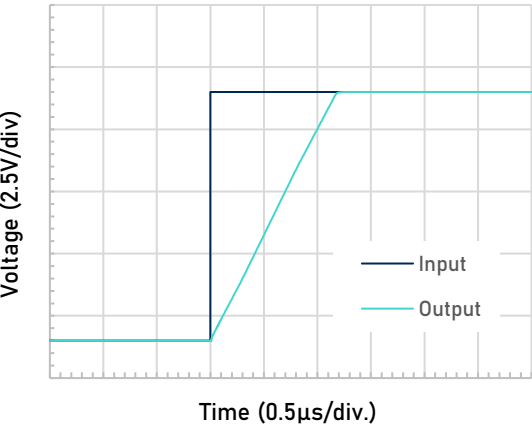
Large-Signal Step Response(Failing)
