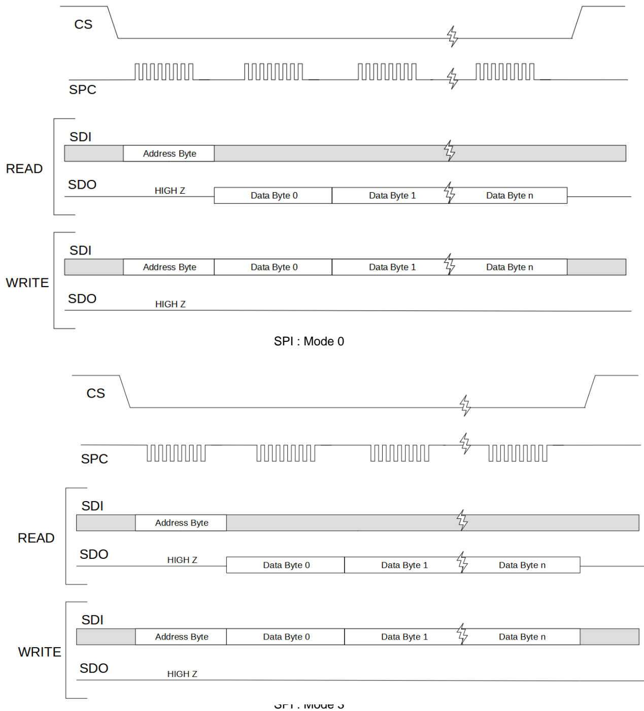
Figure 30. SPI 4-Wire Multi-Byte Read and Write Transactions
