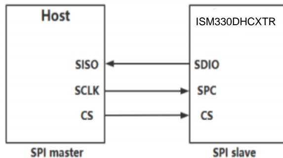
Figure 28. Typical SPI 3-Wire Connection
