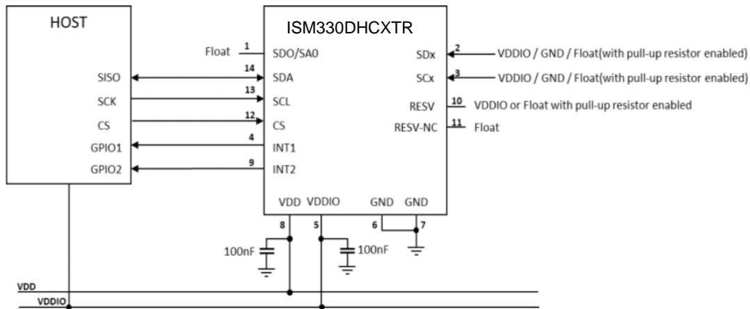
Figure 5. 3-Wire SPI-UI mode
