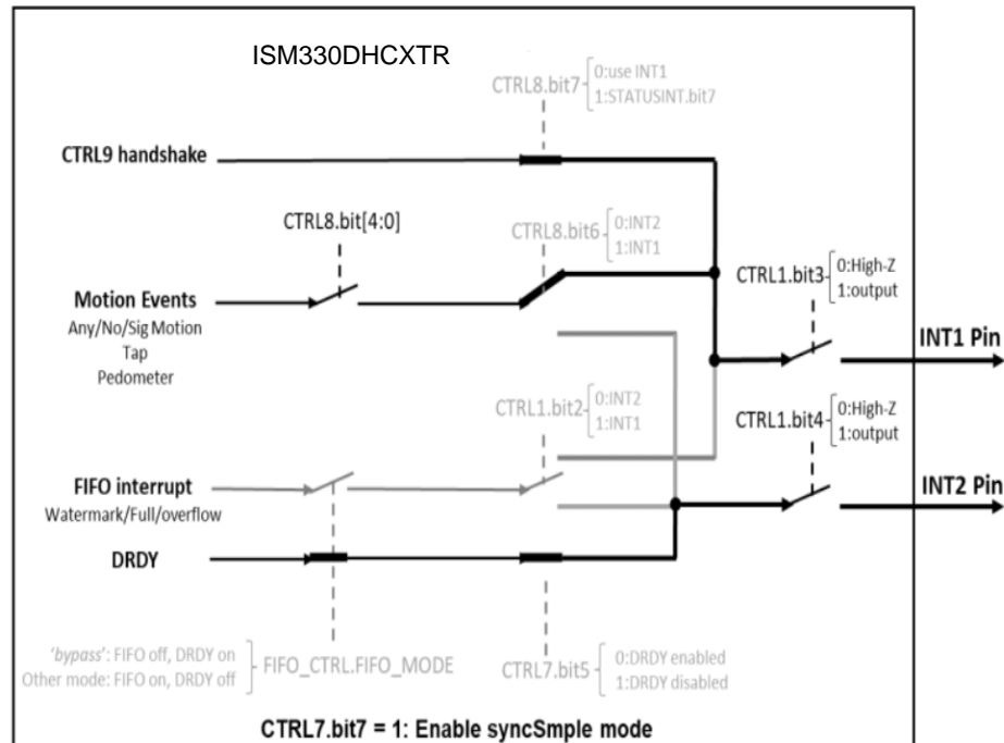
Figure 14. Interrupt Map of SyncSample Mode
