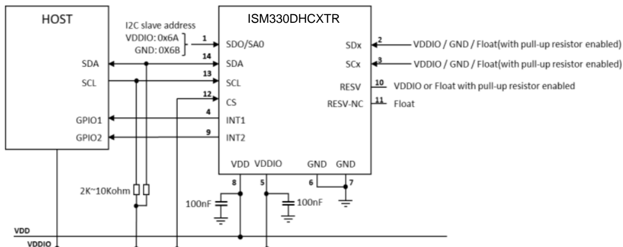
Figure 6. I3C/I2C-UI mode
