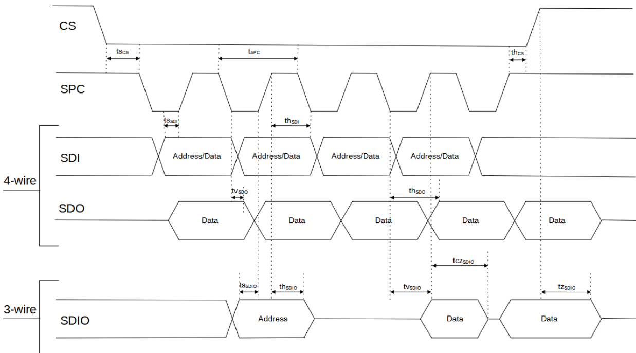
Figure 33. Timing Characteristics for SPI 3- and 4-Wire Interfaces
