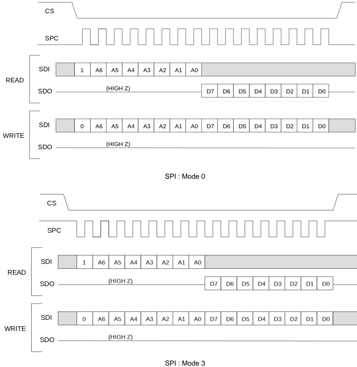
Figure 29. SPI 4-Wire Single Byte Read and Write (Mode 0 and Mode 3)
