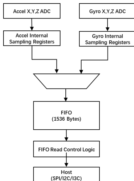
Figure 17. FIFO Data Flow
