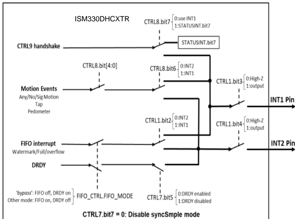
Figure 15. Interrupt Map of Non-SyncSample Mode
