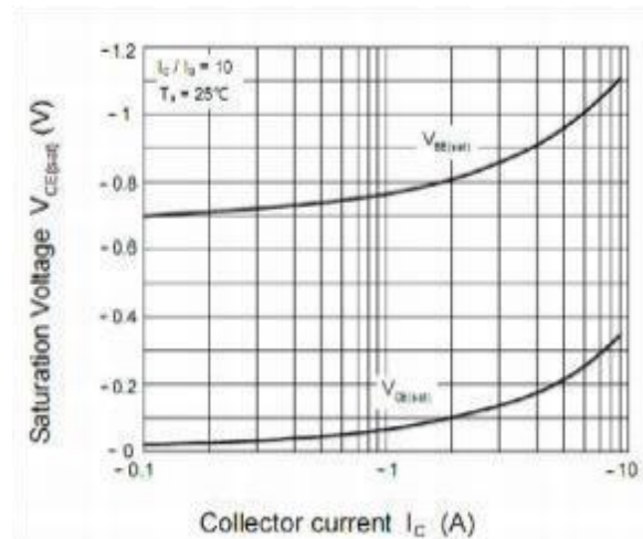
Figure 2 . Saturation Voltage
