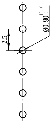
PCB LAYOUT
