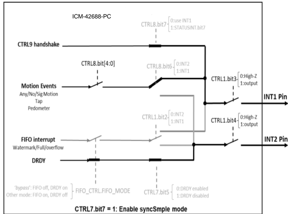
Figure 14. Interrupt Map of SyncSample Mode
