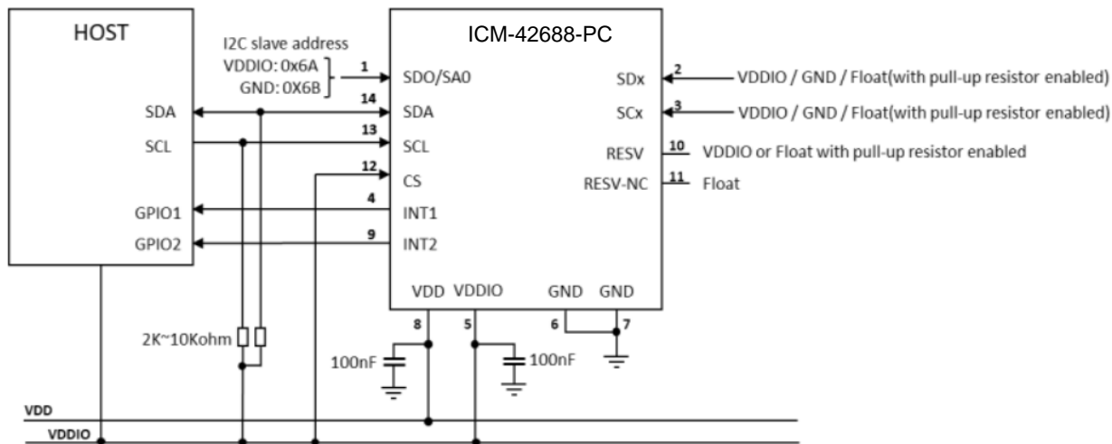
Figure 6. I3C/I2C-UI mode
