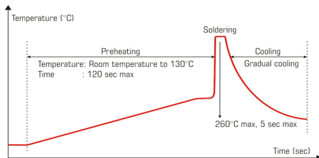
Fig.: Wave-soldering temperature-time profile to recommend
