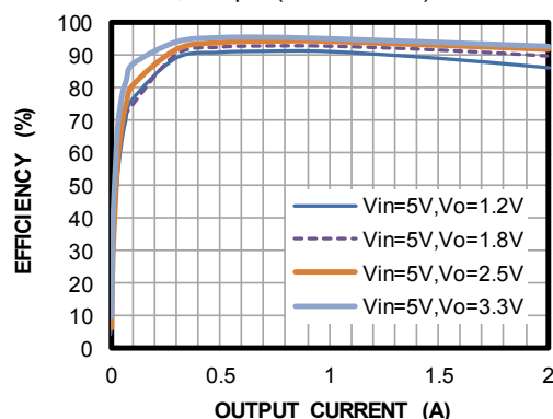
Efficiency vs. Output Current V_{IN}=5V , L=1\mu H (DCR=27mΩ)
