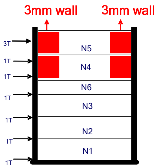
Figure 5—Winding Diagram
