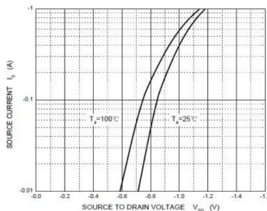
Figure 5: Diode Characteristics
