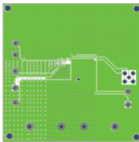
Figure 4—Inner Layer 2
