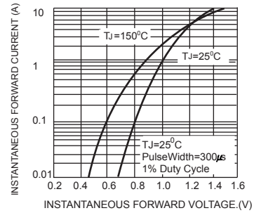
FIG.3 - TYPICAL FORWARD VOLTAGE CHARACTERISTICS PER LEG
