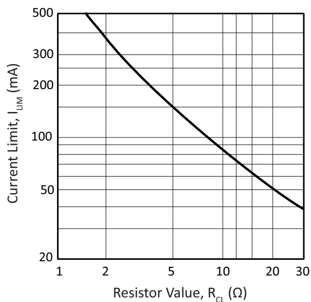
Figure 15: Current Limit
