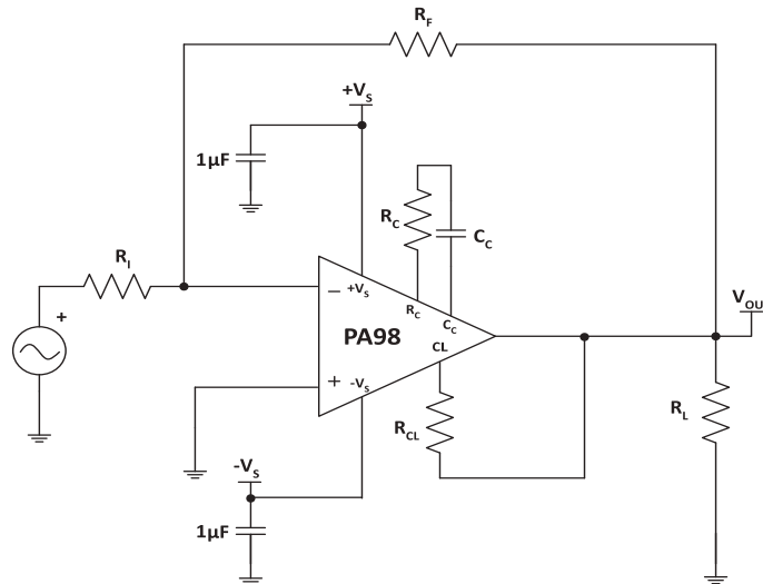
Figure 2: Typical Connections
