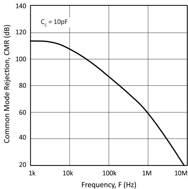
Figure 13: Common Mode Rejection
