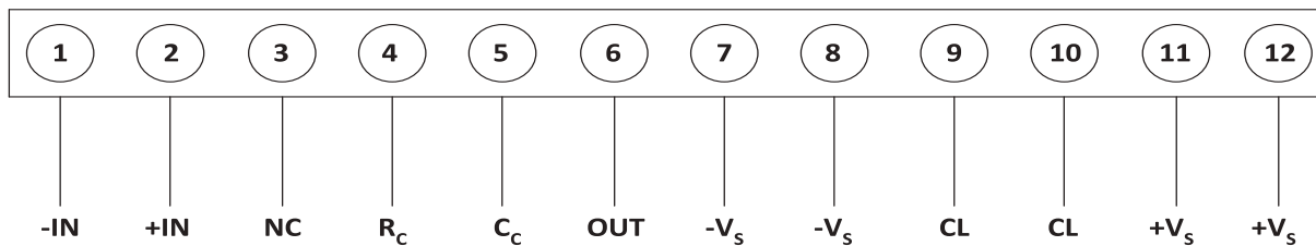
Figure 3: External Connections
