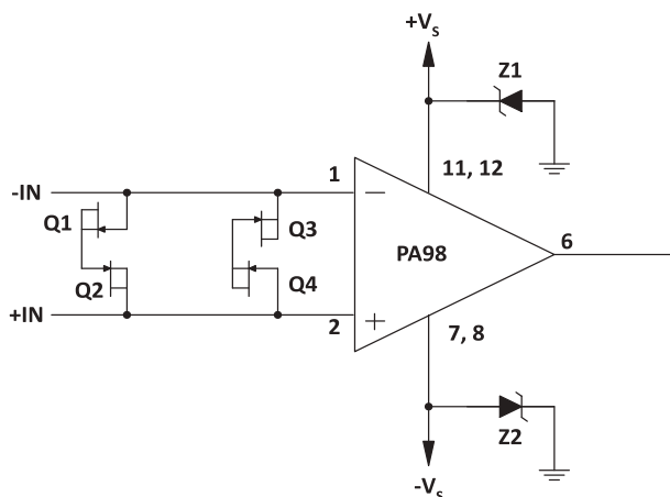
Figure 18: Over Voltage Protection
