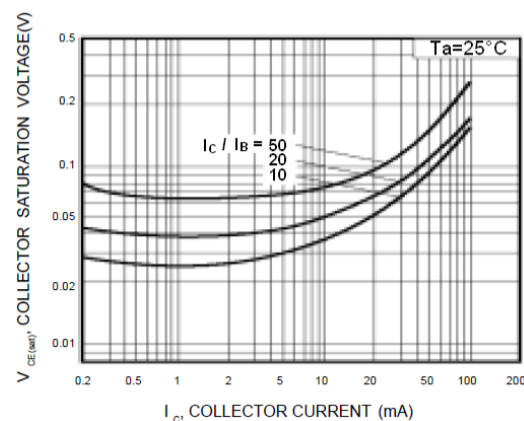
6. Collector-emitter saturation voltage vs. collector current
