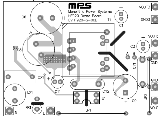
Figure 2: Top Layer
