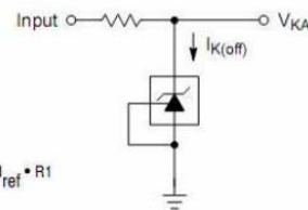
Test Circuit for I_{K(off)}
