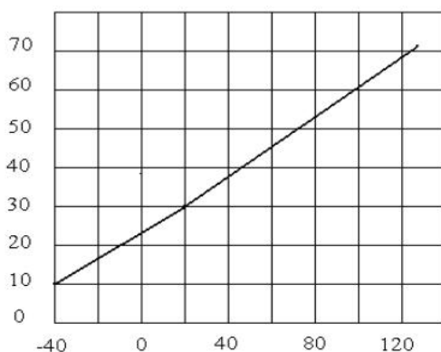
Off-State Cathode Current I_{Koff} (uA) vs. Junction Temperature T_J (°C) U_{Ka}=36V
