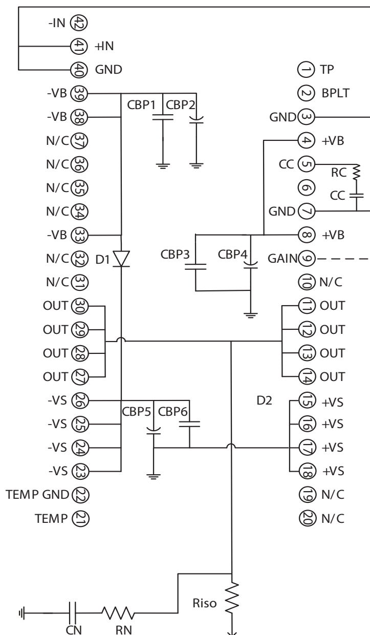
Figure 2: External Connections
