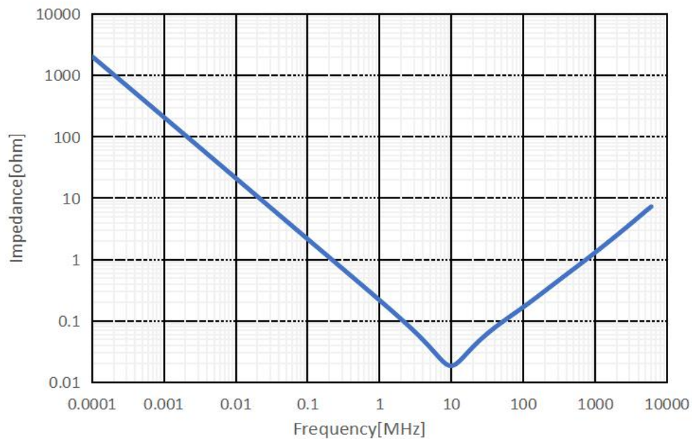
Example of Impedance characteristics
