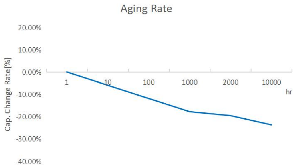
Example of Change Over Time (Aging Characteristics)
