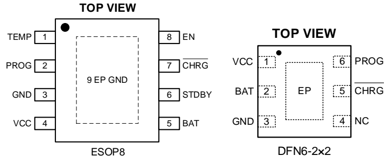
Figure 2. Pin Configuration
