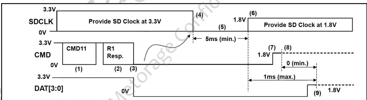
Figure 4-3 Signal Voltage Switch Sequence
