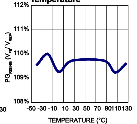
PG Rising Threshold ( V_{FB} Falling) vs. Temperature
