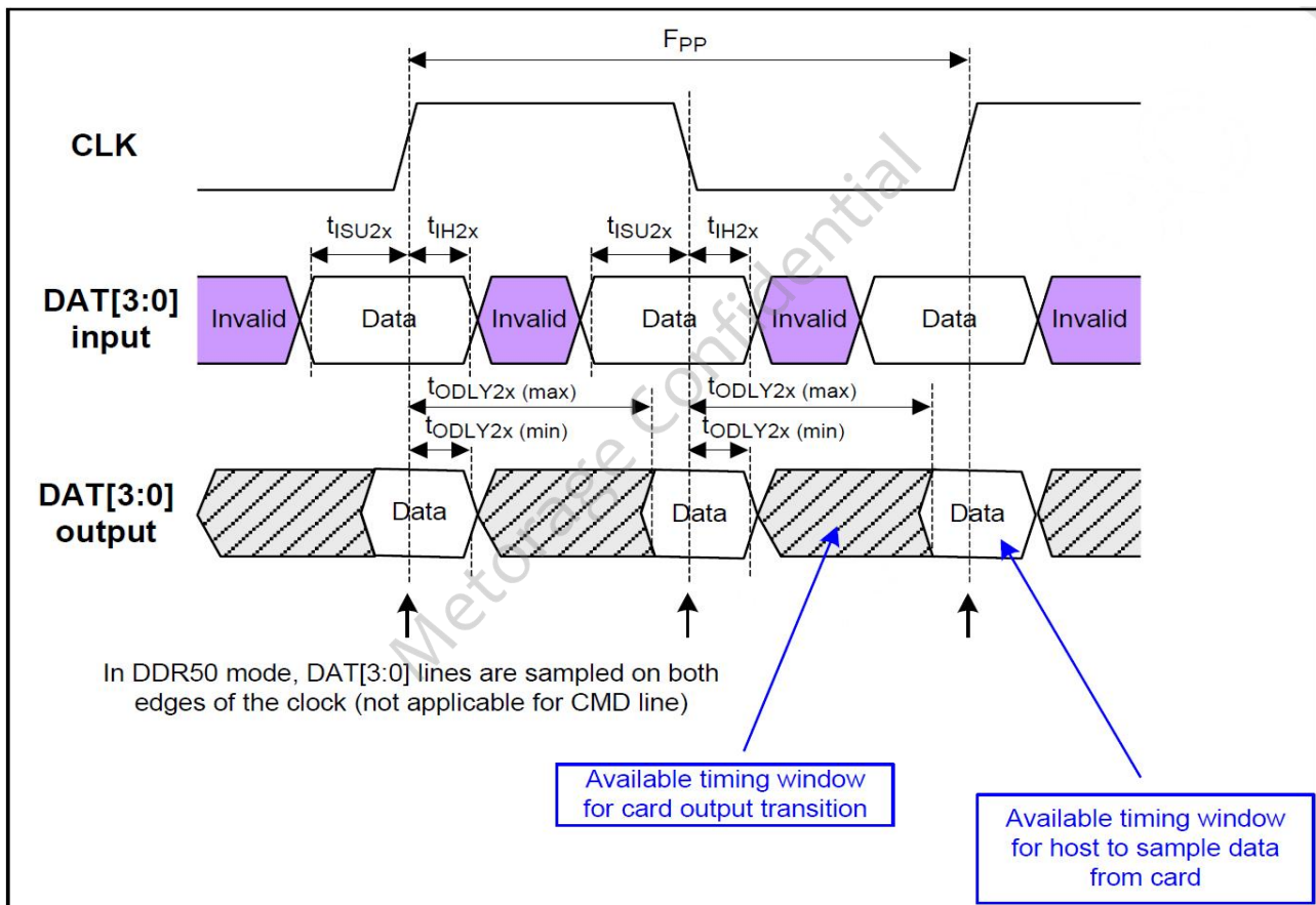
Figure 7- 13 Timing Diagram DAT Inputs/Outputs Referenced to CLK in DDR50 Mode
