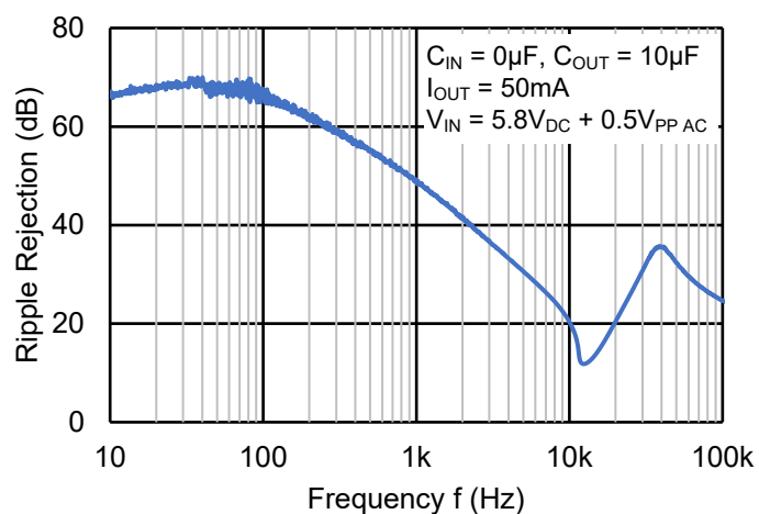
Ripple Rejection
