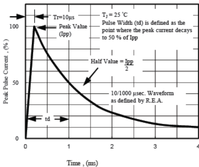
Fig. 5 - Pulse Waveform
