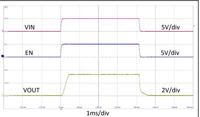
Fig 10. VIN 电源上电、关闭 ( V_{IN} = 5V, I_{OUT} = 5mA )
