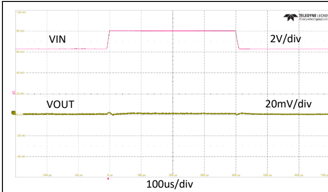
Fig 7. 输入电压瞬变 ( V_{IN} = 4.3V \leftrightarrow 6V )
