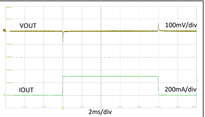
Fig 8. 负载电流瞬变 ( V_{OUT} = 3.3V, I_{OUT} = 1mA \leftrightarrow 300mA )
