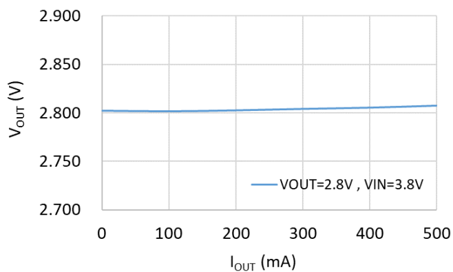
Fig 6. V_{OUT} vs. I_{OUT}
