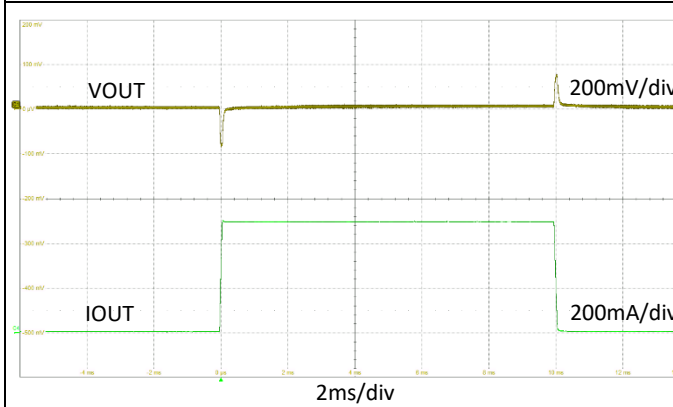
Fig 9. 负载电流瞬变 ( V_{OUT} = 3.3V, I_{OUT} = 1mA \leftrightarrow 500mA )
