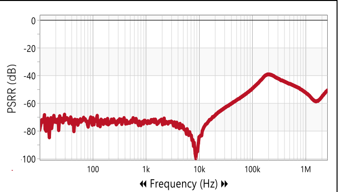
Fig 12. PSRR ( V_{IN} = 4.8V, V_{OUT} = 2.8V, I_{OUT} = 10mA )
