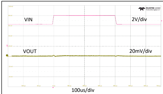
Fig 7. 输入电压瞬变 ( V_{IN} = 4.3V \leftrightarrow 6V )
