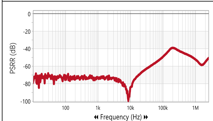
Fig 11. PSRR ( V_{IN} = 4.8V, V_{OUT} = 2.8V, I_{OUT} = 10mA )
