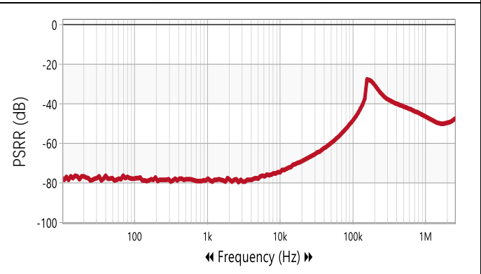
Fig 12. PSRR ( V_{IN} = 4.8V, V_{OUT} = 1.2V, I_{OUT} = 10mA )
