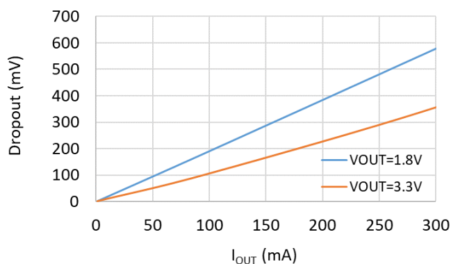
Fig 5. 压差电压 vs. I_{OUT}
