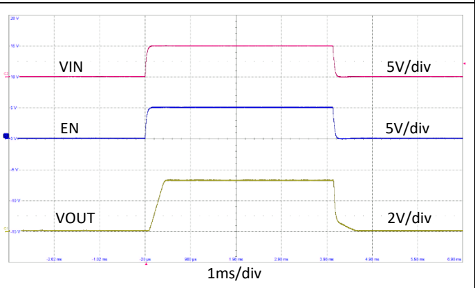
Fig 10. VIN 电源上电、关闭 ( V_{IN} = 5V, I_{OUT} = 5mA )
