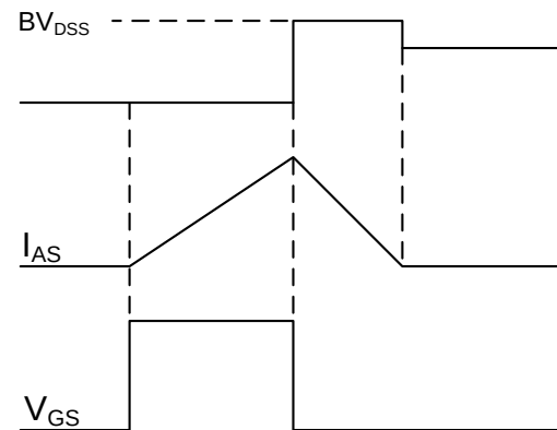
Fig.11 Unclamped Inductive Switching Waveform
