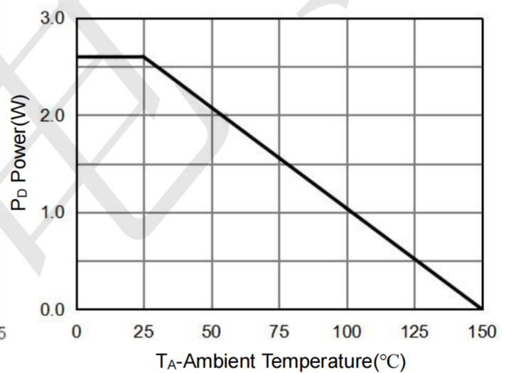
Figure 10 Power Dissipation
