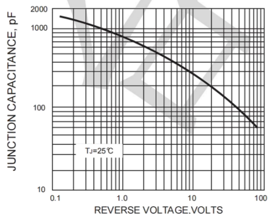
FIG. 5-TYPICAL JUNCTION CAPACITANCE
